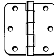
Masonite* Template Hole Pattern
