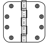
Template Hole Pattern
