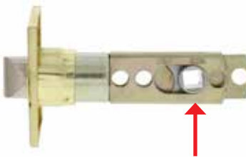
Square drive latches used in residential grade latches
